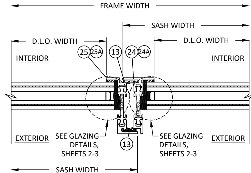
E HORIZONTAL SECTION 15 OUTSIDE GLAZED - ASTRAGAL INSWING DOOR
