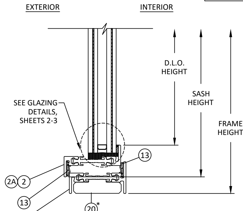
D 13 VERTICAL SECTION OUTSIDE GLAZED - SILL OUTSWING DOOR
