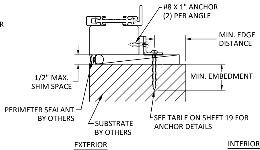
E 20 VERTICAL SECTION SILL - 3/4" X 3/4" ALUMINUM/STEEL ANGLE OUTSIDE GLAZED
