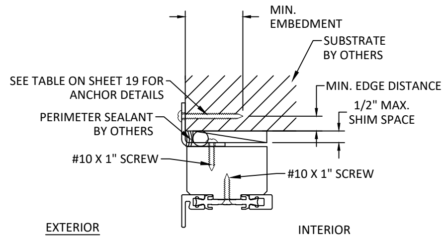
A 20 VERTICAL SECTION HEAD - ALUMINUM/STEEL BENT EXT. CLIP JAMB AND SILL SIMILAR INSIDE GLAZED
