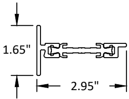
24 SASH BRONZE
