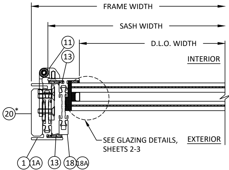
D HORIZONTAL SECTION 15 OUTSIDE GLAZED - HINGE JAMB INSWING DOOR
