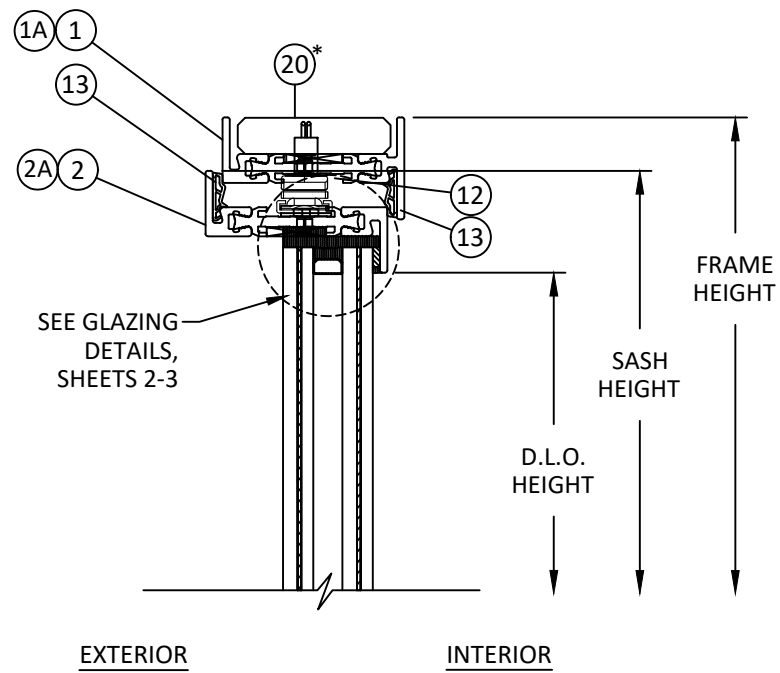
C 13 VERTICAL SECTION OUTSIDE GLAZED - HEAD OUTSWING DOOR
