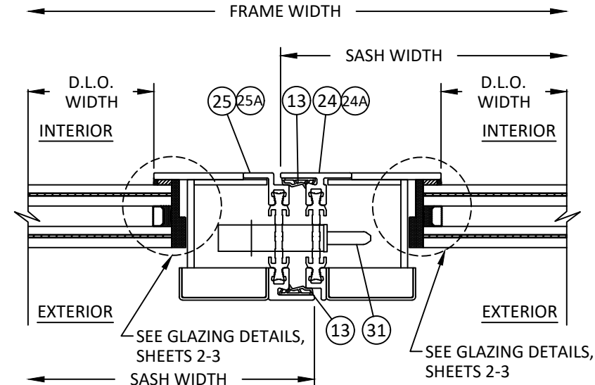
F HORIZONTAL SECTION 15 OUTSIDE GLAZED - LOCK BOX INSWING DOOR
