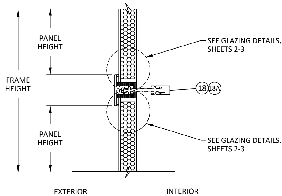
F 12 VERTICAL SECTION INSIDE GLAZED - MIDRAIL
