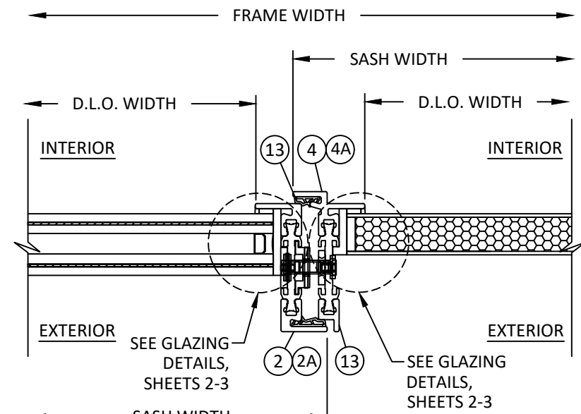
F 17 HORIZONTAL SECTION OUTSIDE GLAZED - MEETING STILE OUTSWING DOOR
