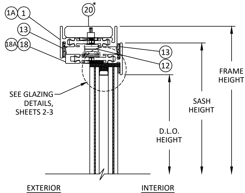
C 12 VERTICAL SECTION OUTSIDE GLAZED - HEAD INSWING DOOR
