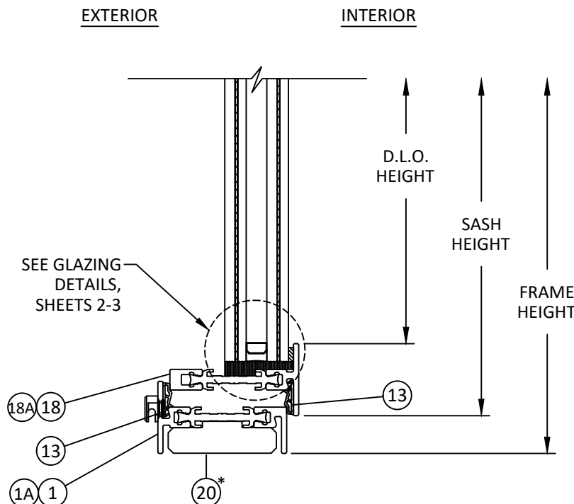
D 12 VERTICAL SECTION OUTSIDE GLAZED - SILL INSWING DOOR
