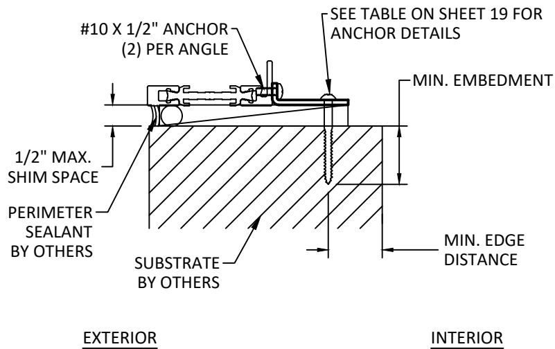
A 22 VERTICAL SECTION SILL - 1/2" X 1-4/5" ALUMINUM/STEEL ANGLE OUTSIDE GLAZED
