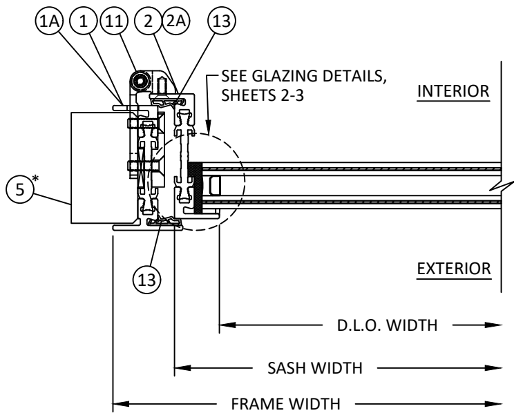
A HORIZONTAL SECTION 15 INSIDE GLAZED - HINGE JAMB INSWING DOOR
