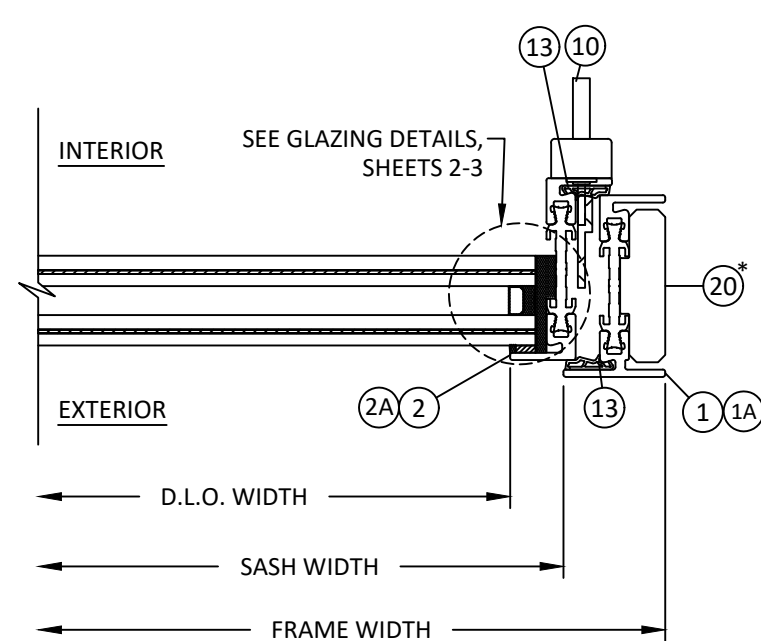
A 17 HORIZONTAL SECTION INSIDE GLAZED - LOCK JAMB INSWING DOOR
