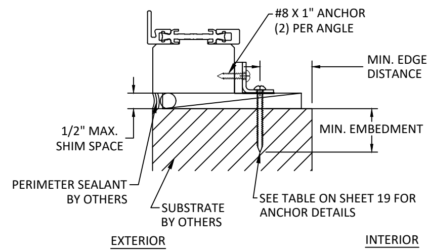
F 20 VERTICAL SECTION SILL - 3/4" X 3/4" ALUMINUM/STEEL ANGLE INSIDE GLAZED
