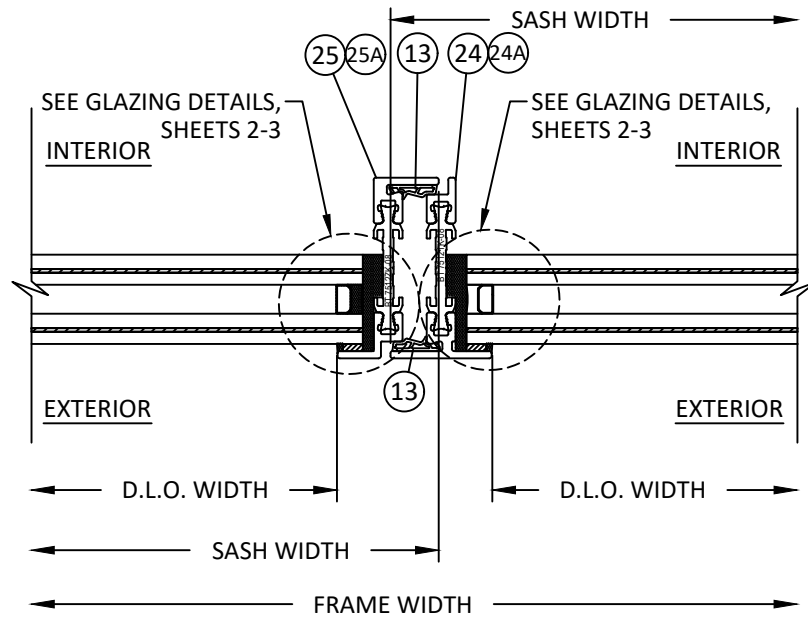
B HORIZONTAL SECTION 15 INSIDE GLAZED - ASTRAGAL INSWING DOOR
