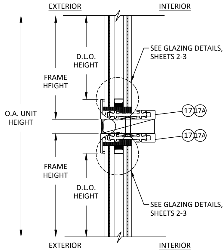
C 18 VERTICAL SECTION TRANSOM TO SIDELITE MULLION
