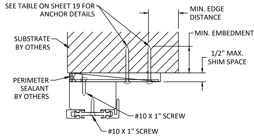
E 21 VERTICAL SECTION HEAD - ALUMINUM/STEEL FLAT CLIP JAMB SIMILAR OUTSIDE GLAZED
