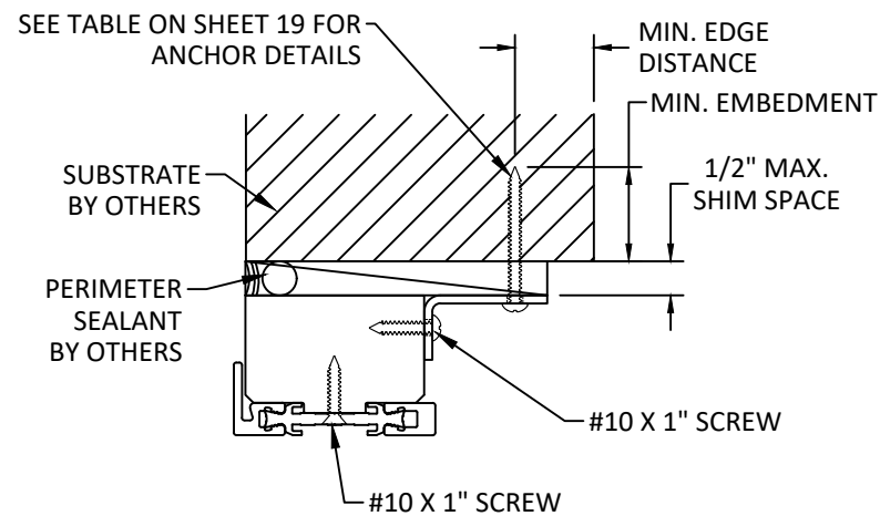
D 21 VERTICAL SECTION HEAD - ALUMINUM/STEEL BENT INT. CLIP JAMB SIMILAR INSIDE GLAZED
