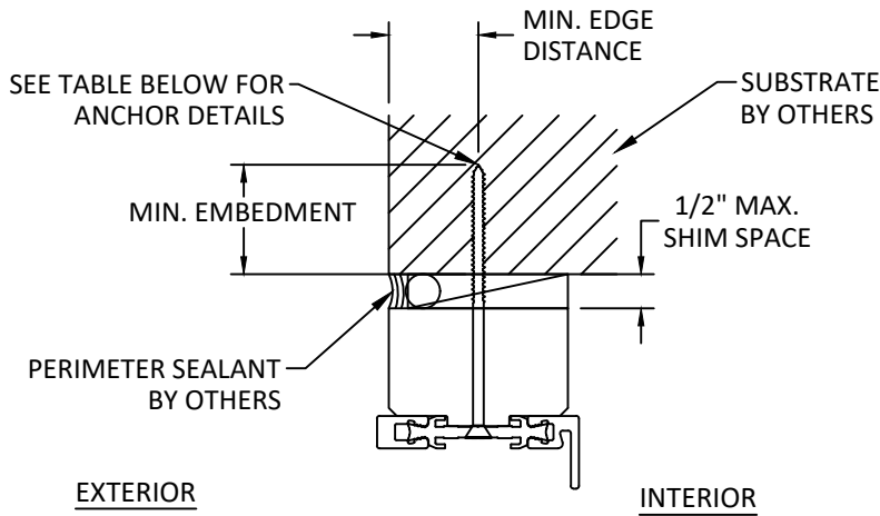
B 19 VERTICAL SECTION HEAD - THROUGH FRAME JAMB AND SILL SIMILAR OUTSIDE GLAZED
