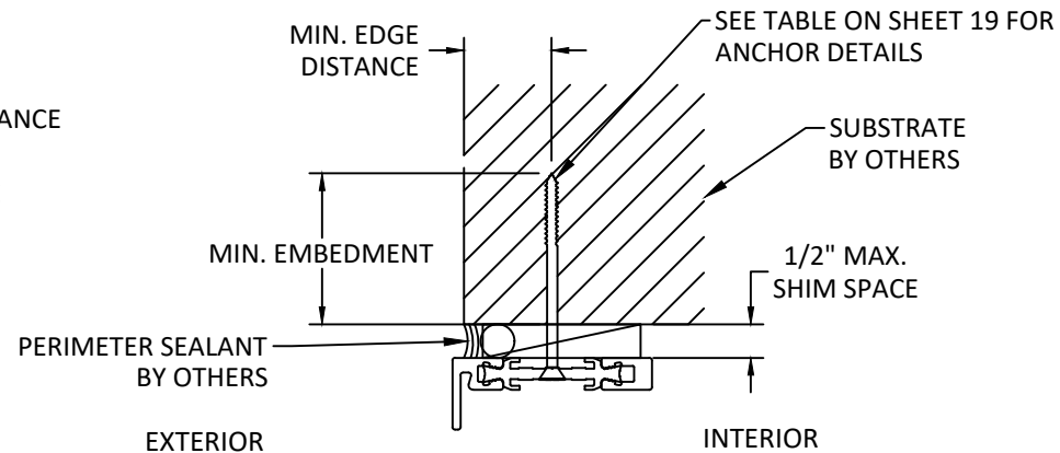
C 20 VERTICAL SECTION HEAD - THROUGH FRAME JAMB AND SILL SIMILAR INSIDE GLAZED
