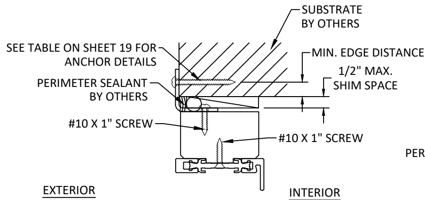
B 20 VERTICAL SECTION HEAD - ALUMINUM/STEEL BENT EXT. CLIP JAMB AND SILL SIMILAR OUTSIDE GLAZED
