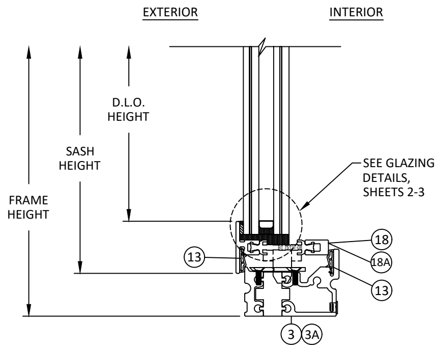
B 13 VERTICAL SECTION INSIDE GLAZED - SILL OUTSWING DOOR
