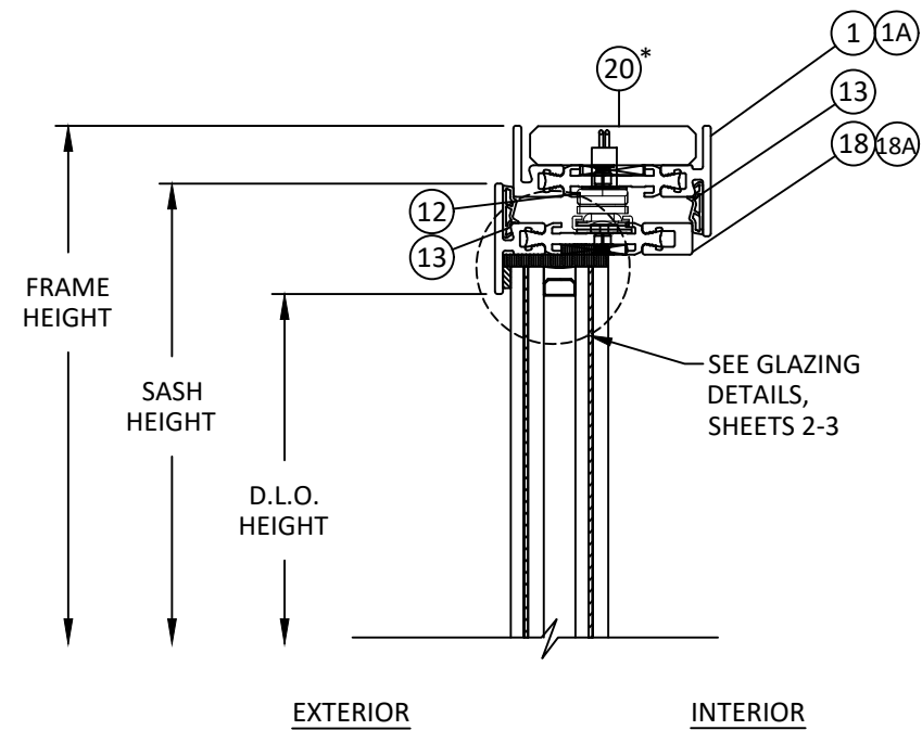
A 13 VERTICAL SECTION INSIDE GLAZED - HEAD OUTSWING DOOR
