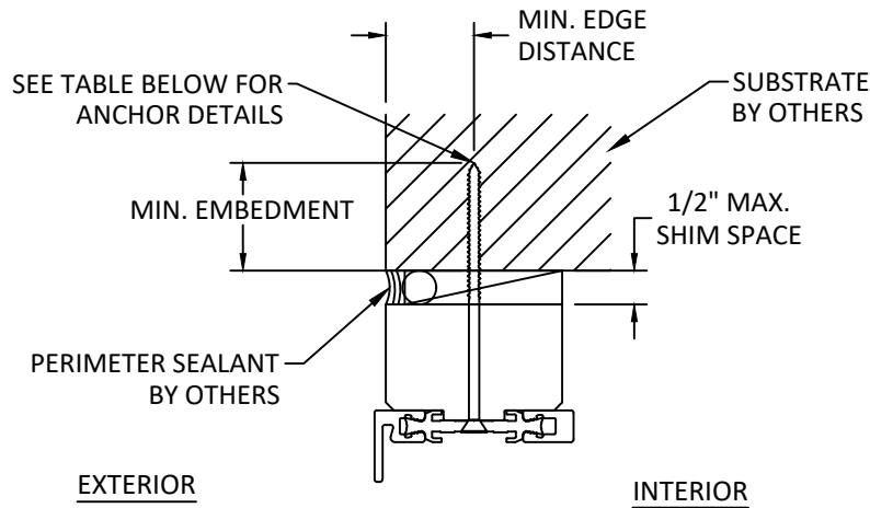
A 19 VERTICAL SECTION HEAD - THROUGH FRAME JAMB AND SILL SIMILAR INSIDE GLAZED
