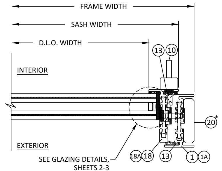
D 17 HORIZONTAL SECTION OUTSIDE GLAZED - LOCK JAMB INSWING DOOR
