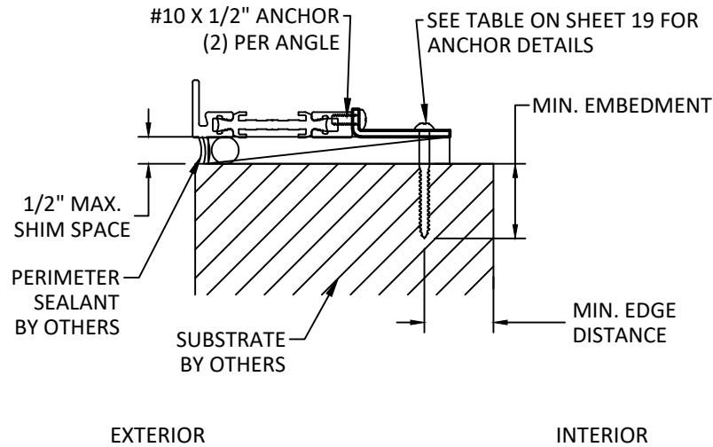
B 22 VERTICAL SECTION SILL - 1/2" X 1-4/5" ALUMINUM/STEEL ANGLE INSIDE GLAZED
