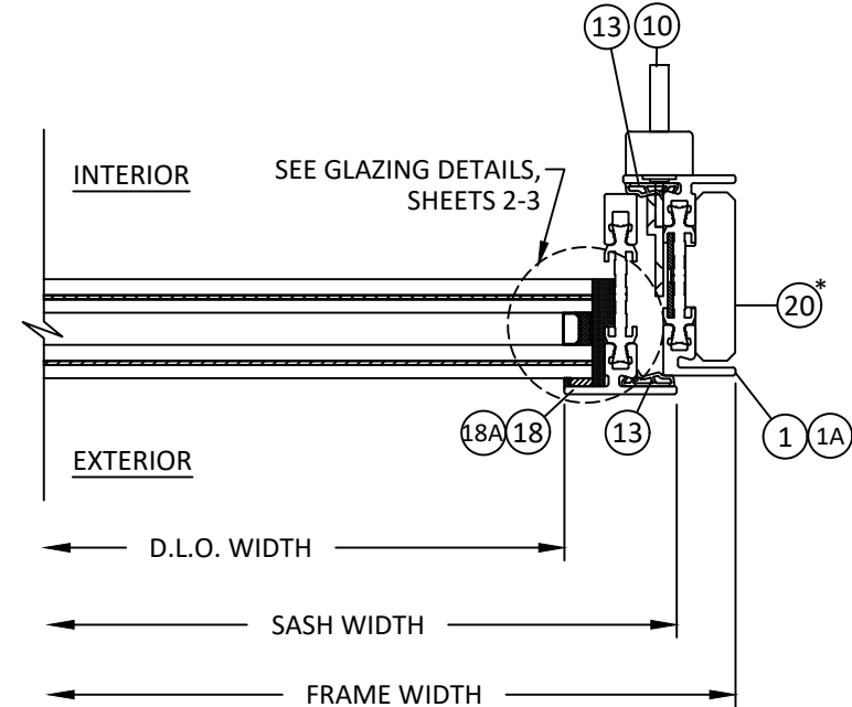
B 17 HORIZONTAL SECTION INSIDE GLAZED - LOCK JAMB OUTSWING DOOR
