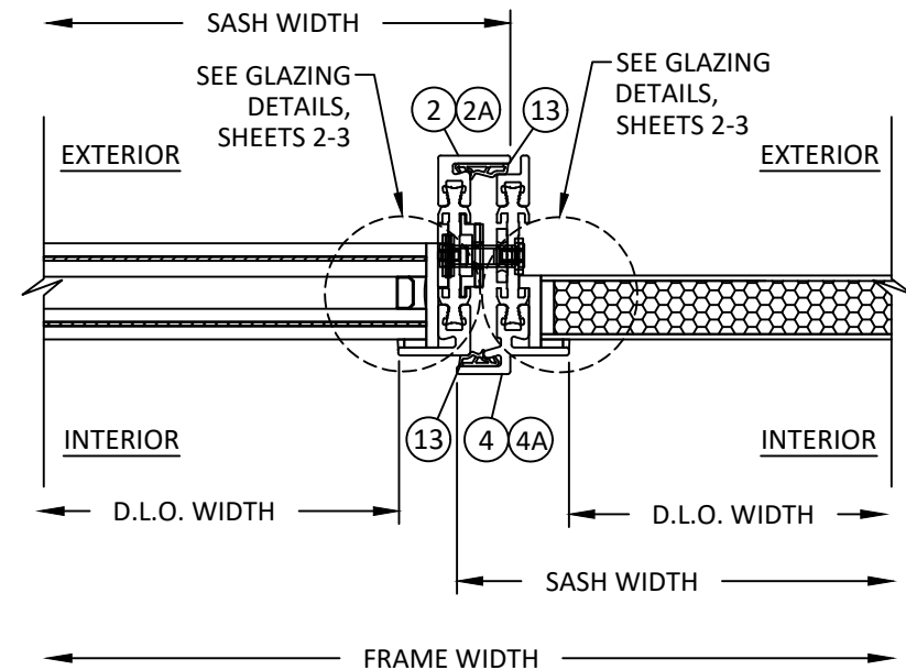
C 17 HORIZONTAL SECTION INSIDE GLAZED - MEETING STILE INSWING DOOR
