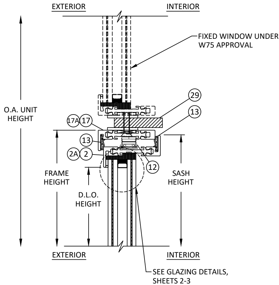
B 18 VERTICAL SECTION 1/2" X 2-1/2" MULLION DETAIL
