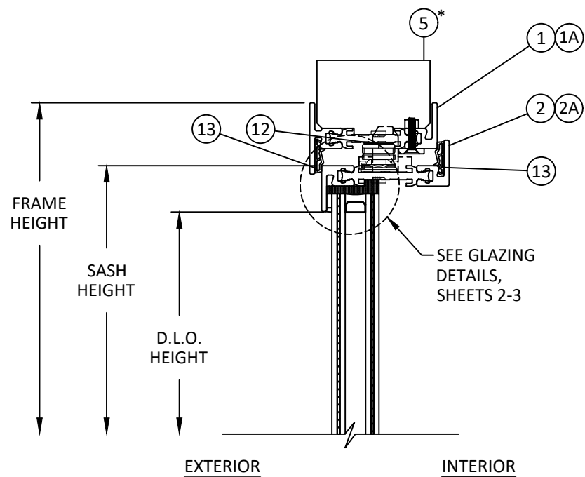
A 12 VERTICAL SECTION INSIDE GLAZED - HEAD INSWING DOOR
