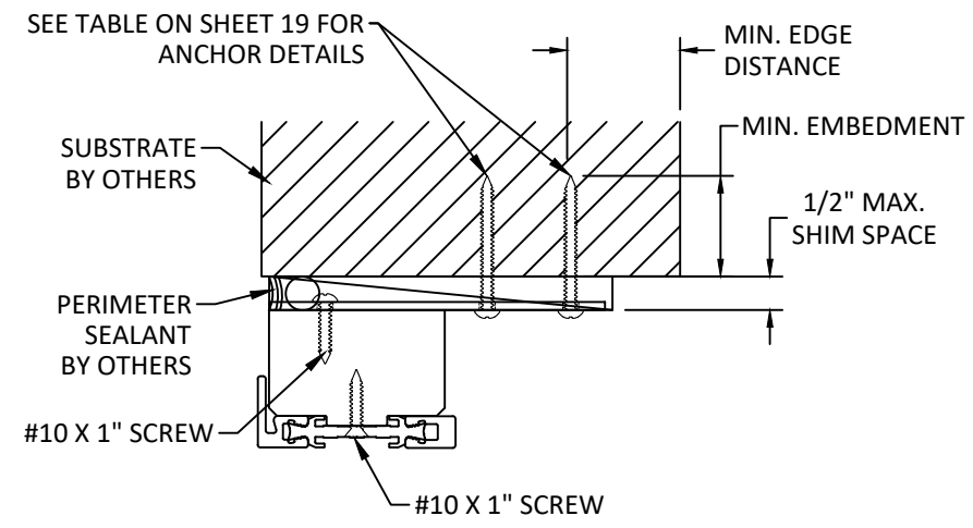
F 21 VERTICAL SECTION HEAD - ALUMINUM/STEEL FLAT CLIP JAMB SIMILAR INSIDE GLAZED
