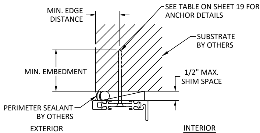
D 20 VERTICAL SECTION HEAD - THROUGH FRAME JAMB AND SILL SIMILAR OUTSIDE GLAZED
