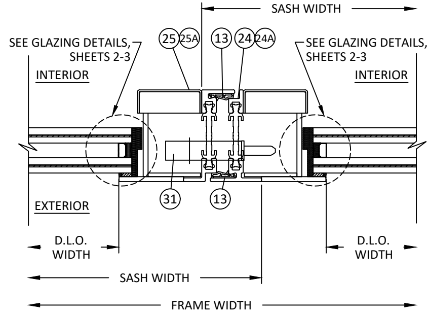
C HORIZONTAL SECTION 15 INSIDE GLAZED - LOCK BOX INSWING DOOR
