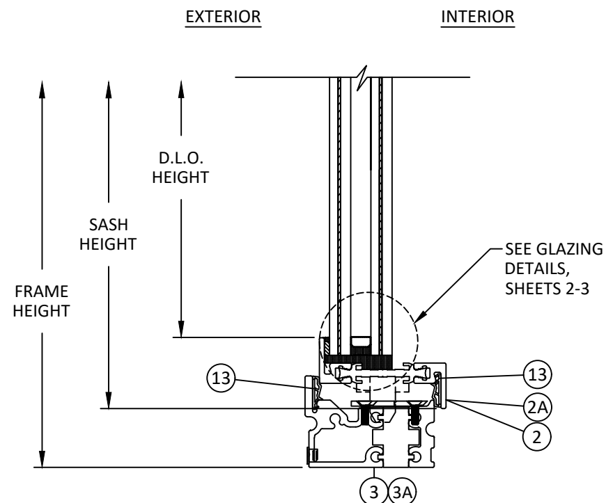
B 12 VERTICAL SECTION INSIDE GLAZED - SILL INSWING DOOR
