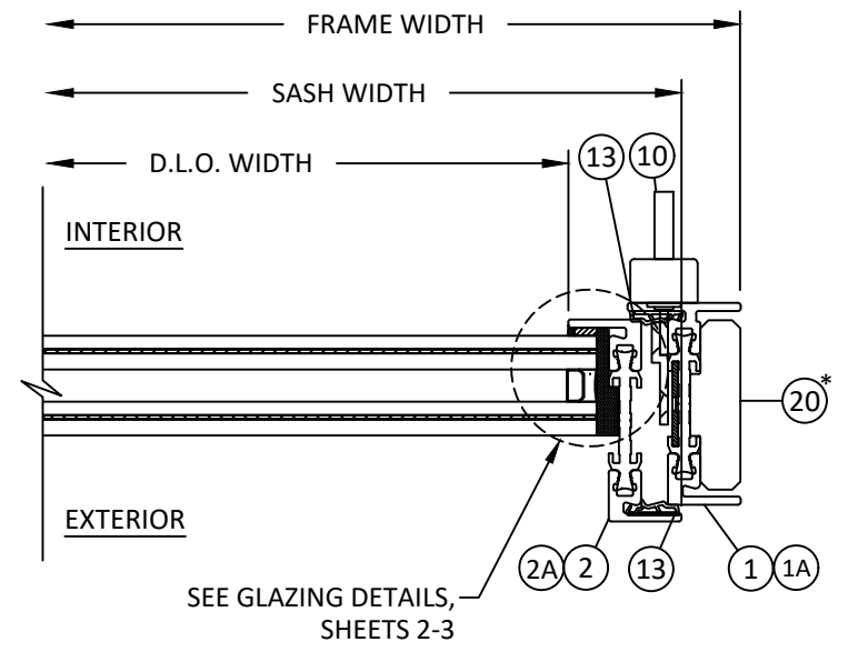
E 17 HORIZONTAL SECTION OUTSIDE GLAZED - LOCK JAMB OUTSWING DOOR
